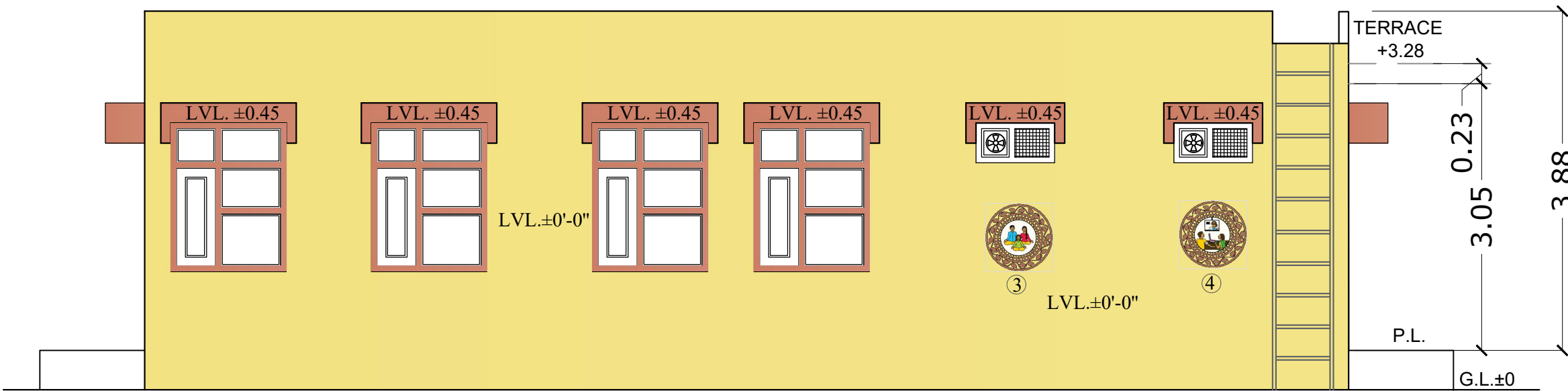
REAR ELEVATION
